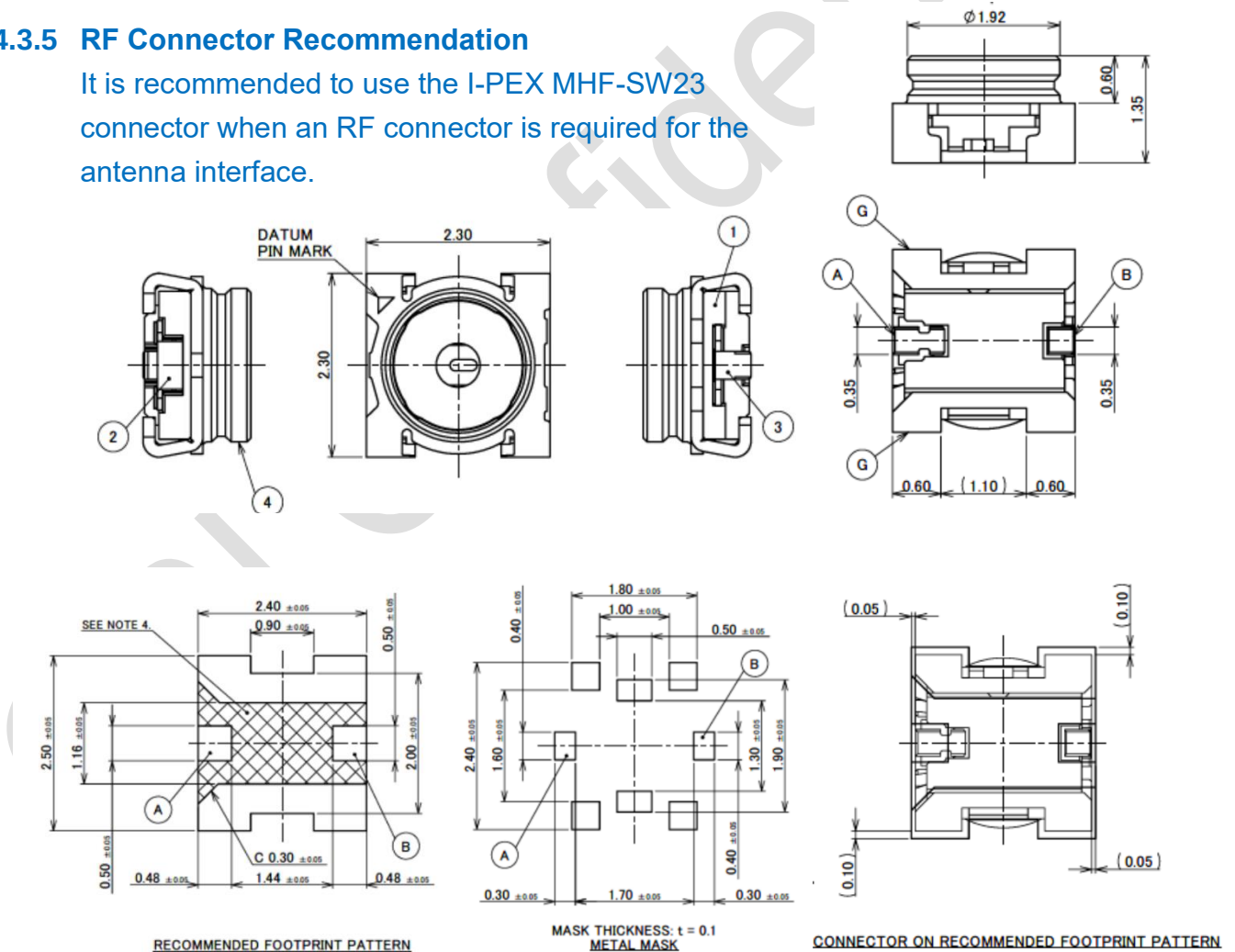
Figure : Dimensions of the Receptacle (Unit:mm)
