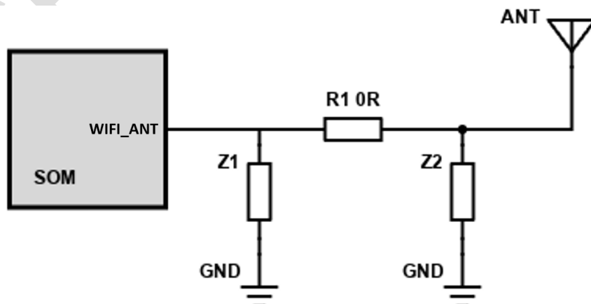
Figure : RF Antenna Reference Design
